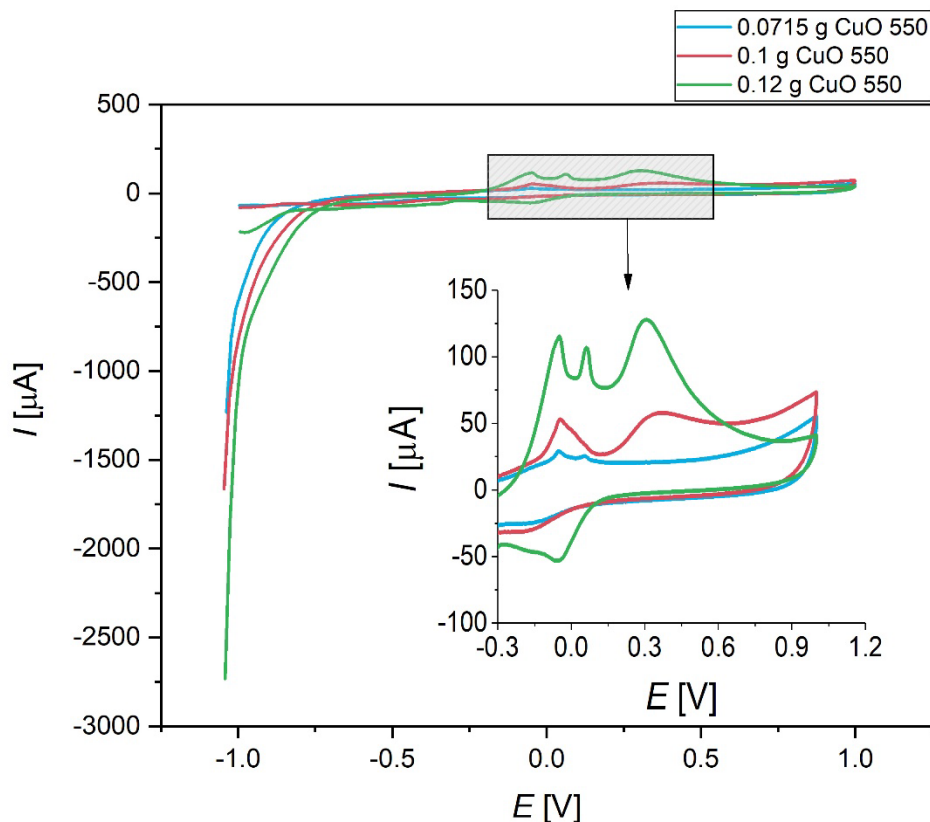
Figure 7 Cyclic voltammetry in 10 \mu\text{M} insulin in PBS (pH=7) on SPCE electrodes modified with MWCNTs and various amounts of CuO 550 fibers at a scan rate of 100 \text{mV}\cdot\text{s}^{-1} .
